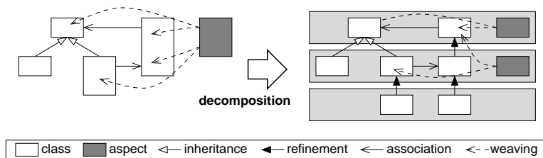
Fig. 3. Feature-driven decomposition of aspect-oriented architectures (features are depicted light-gray).
