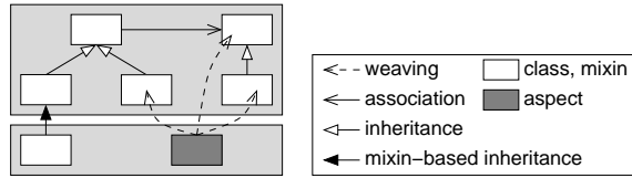
Fig. 4. Aspectual mixin layers.
