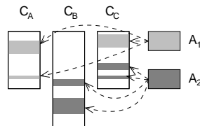
Fig. 2. Two aspects extend three classes.
