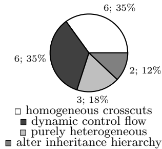
Fig. 18. Applications of aspects (number).
