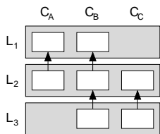
Fig. 1. Stack of three mixin layers.
