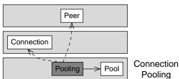
Fig. 10. Connection pooling AML.
