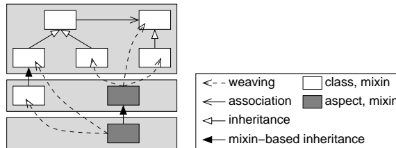
Fig. 5. Aspect refinement.
