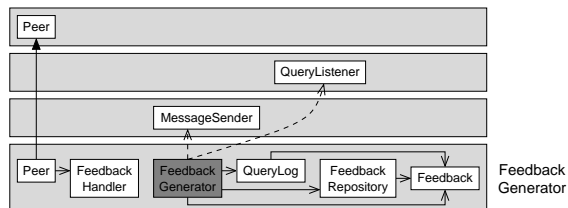
Fig. 7. Feedback generator AML.
