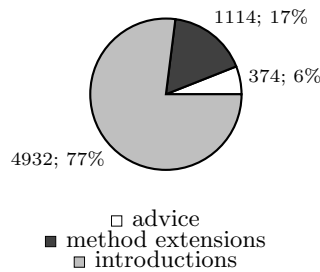
Fig. 17. Static and dynamic crosscutting (LOC).
